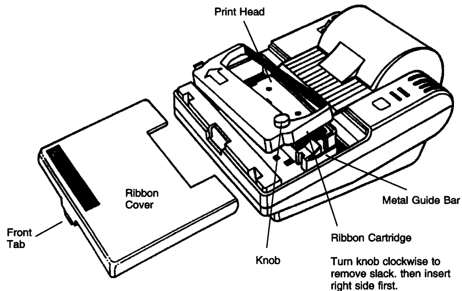
Figure 1-4. Installing the Ribbon Cartridge
