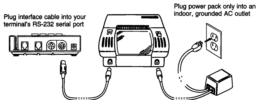
Figure 1-3. Printer Connections
